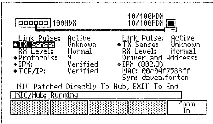
Figure 6-5. Ethernet Expert-T Autotest Sample Results
